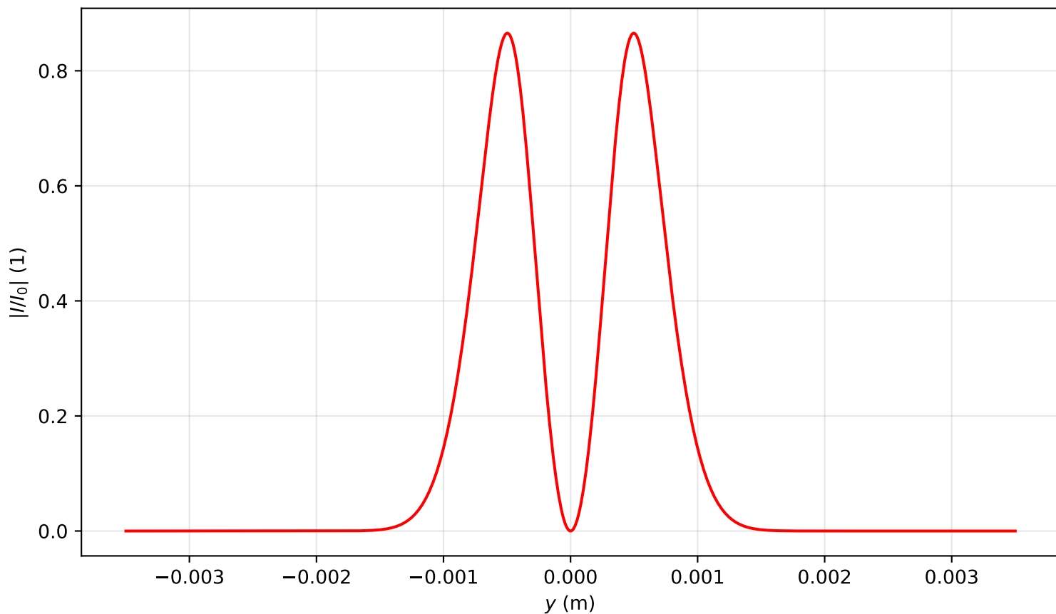
Intensity profile I(x=0, y, z=0.239)/I_0 , P_{in}=3.0P_{cr} , artificial time
